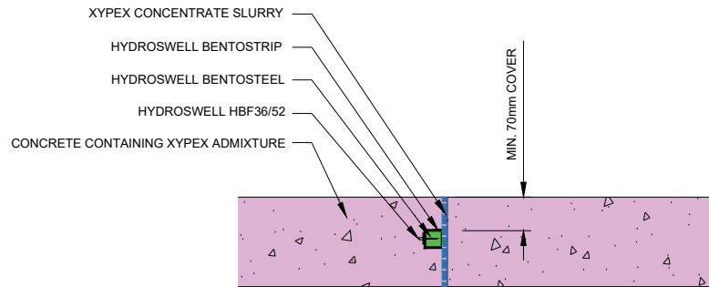
NEW SLAB CONSTRUCTION JOINT
