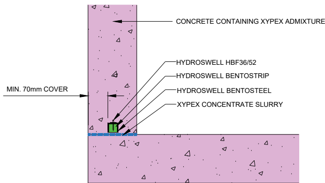
KICKERLESS CONSTRUCTION
