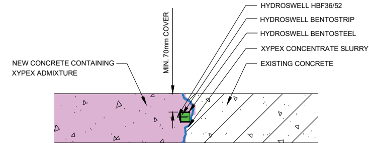
NEW TO EXISTING CONSTRUCTION JOINT
