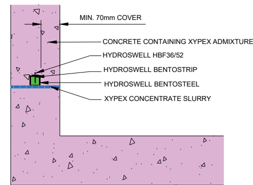
KICKER CONSTRUCTION
